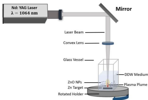
Figure 4: laser ablation (LA) procedure
