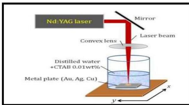
Figure 3: Pulsed Laser Ablation in Liquids (PLAL).
